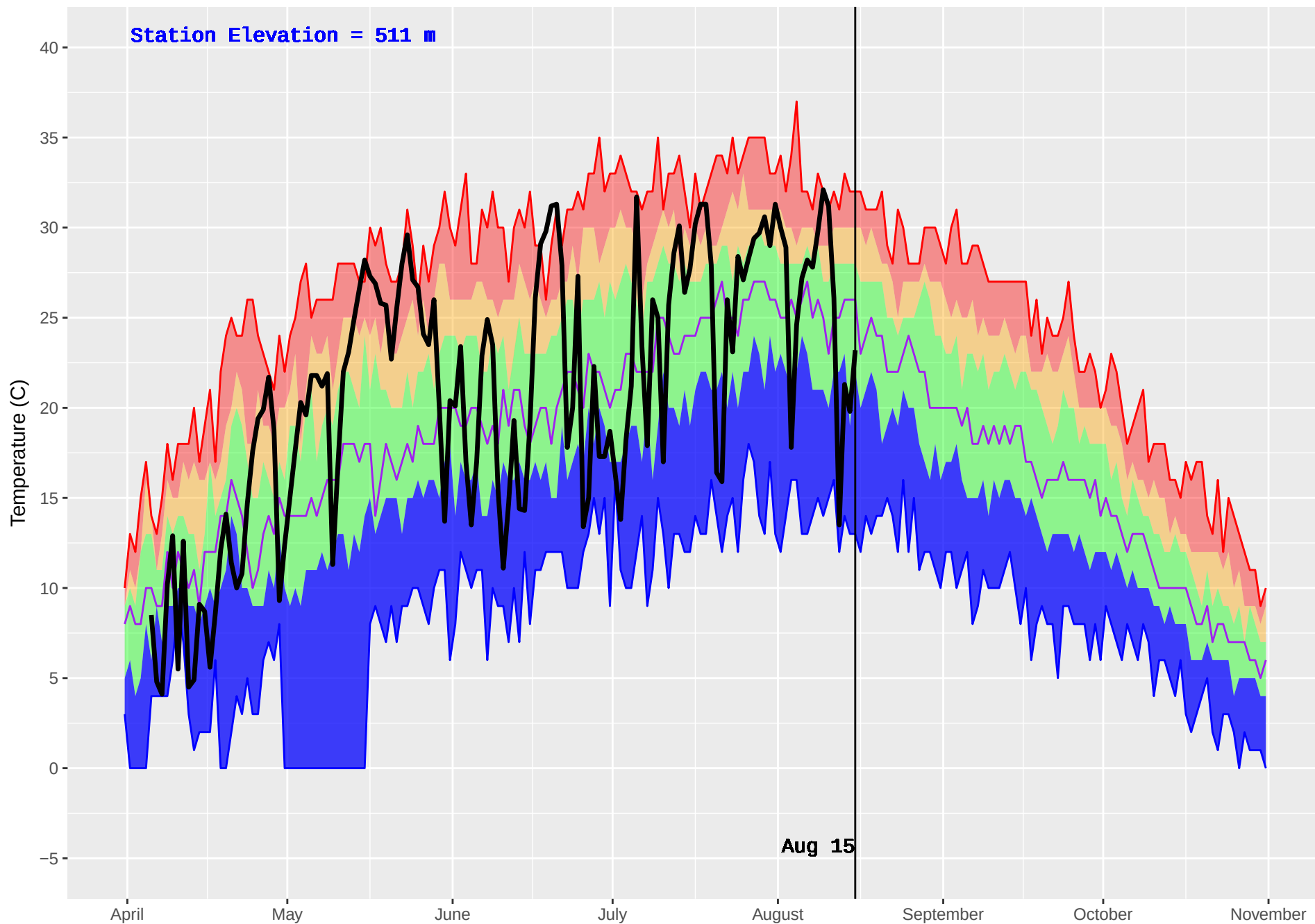
SEYMOUR ARM (344) : Historical (1981–2016) and Current (2018) Daily Temperature
